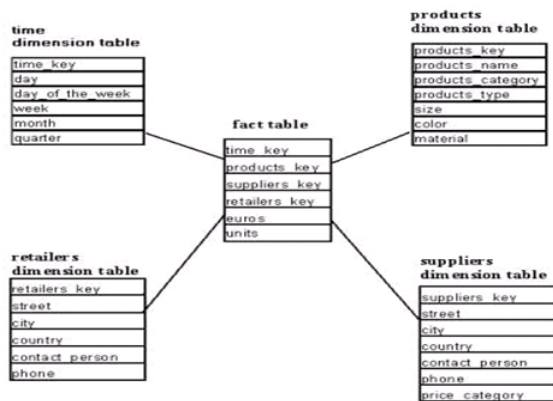
Fig. 2: DW Star Schema Design
