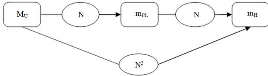
Fig. 2. Relationships for three basic ratios Notes: 1. M_U/m_{PL} = m_{PL}/m_H = (c^5/(2hGH^2))^{1/2} = 6.05 \times 10^{60} = N 2. M_U/m_H = c^5/(2hGH^2) = 36.60 \times 10^{120} = N^2
