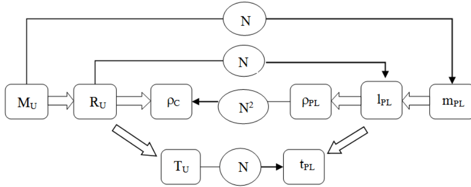
Fig. 1. Black hole relationships Notes: 1. N = Constant for any two black holes 2. Line points to ratio denominator; Bold arrow points to dependent equation 3. M_U/m_{PL} = R_U/l_{PL} = T_U/t_{PL} = N ; \rho_{PL}/\rho_C = N^2
